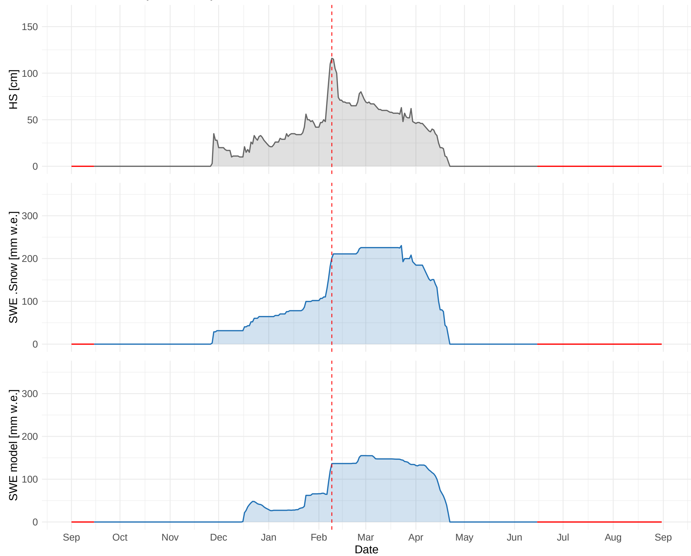
HSD_CH_ZER_MAN (1638 m a.s.l.) – 1983 to 1984
