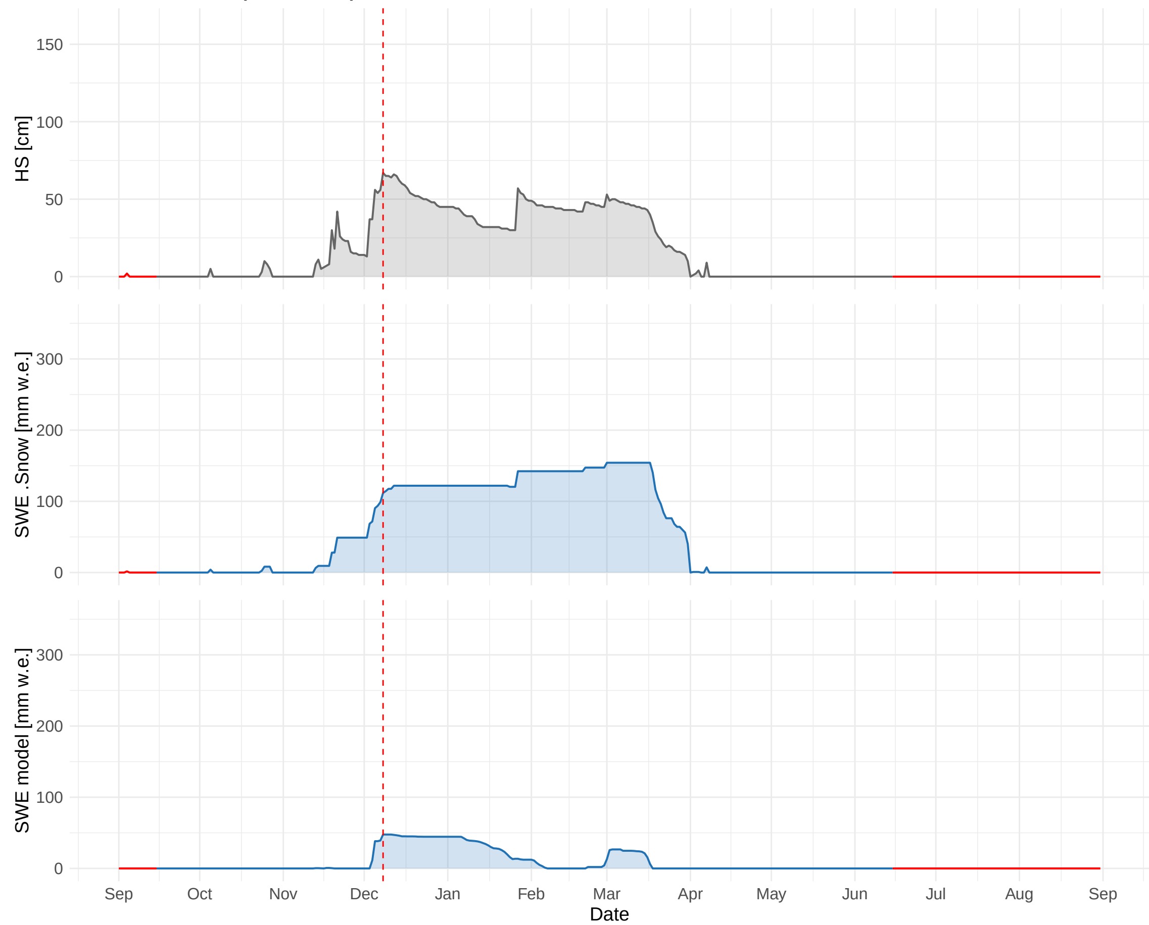
HSD_CH_ZER_MAN (1638 m a.s.l.) – 1992 to 1993
