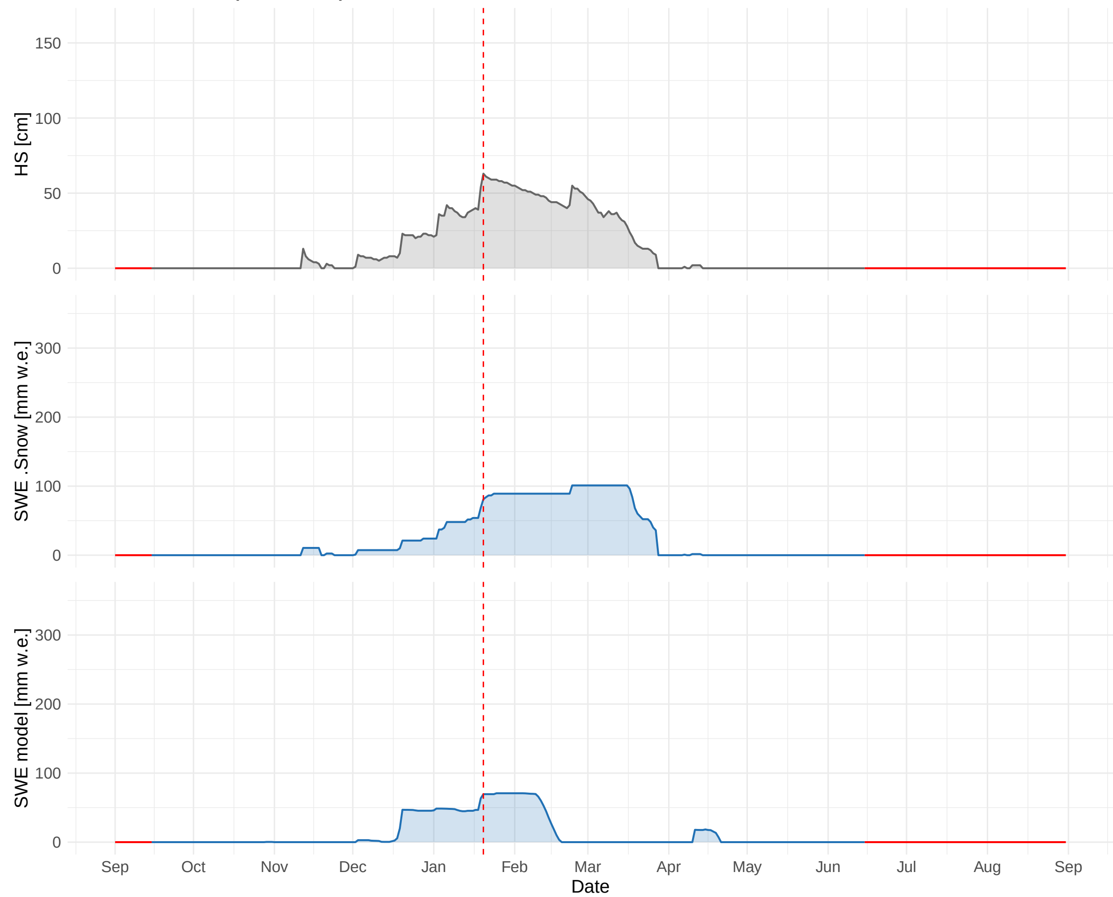
HSD_CH_ZER_MAN (1638 m a.s.l.) – 1997 to 1998
