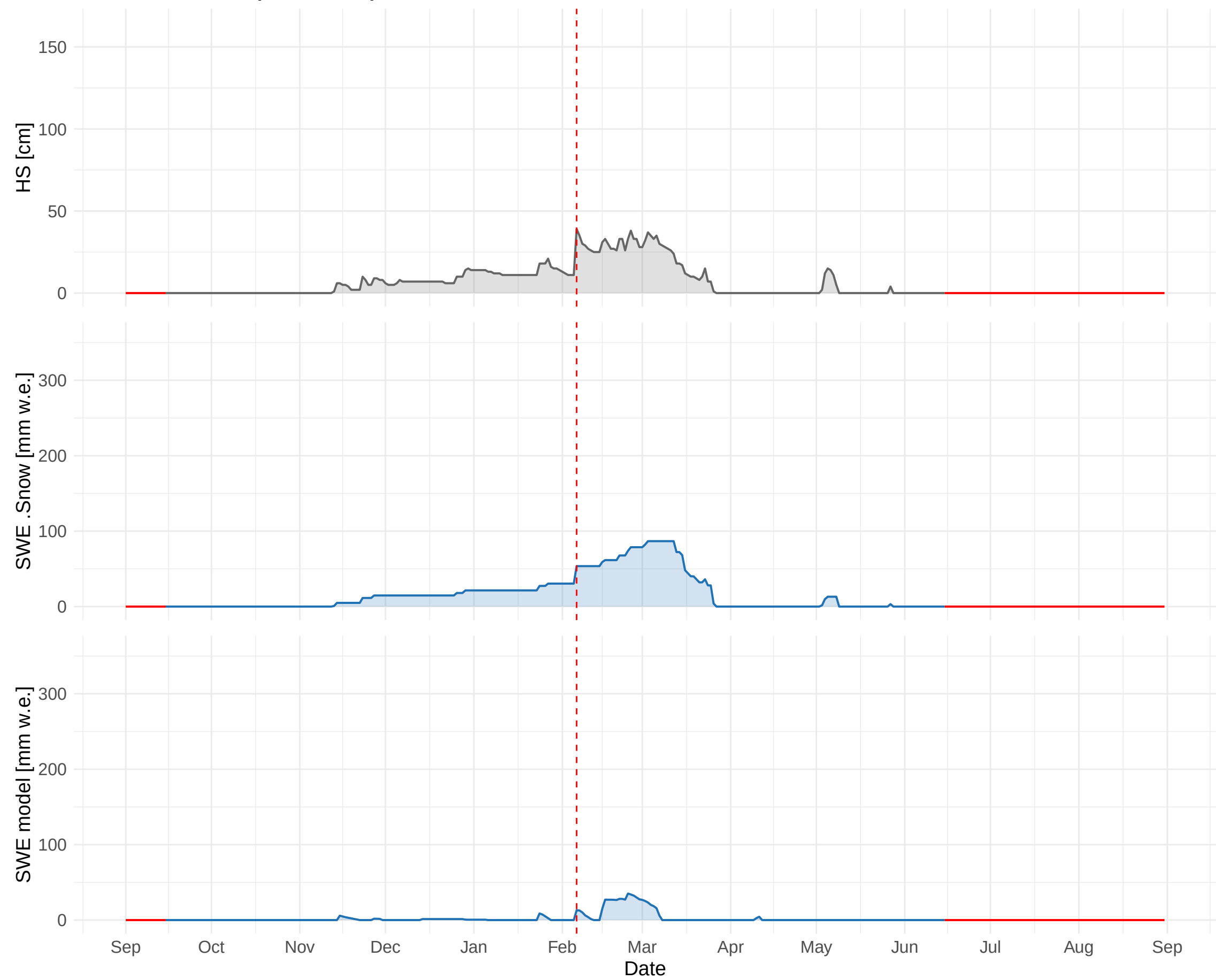
HSD_CH_ZER_MAN (1638 m a.s.l.) – 2001 to 2002
