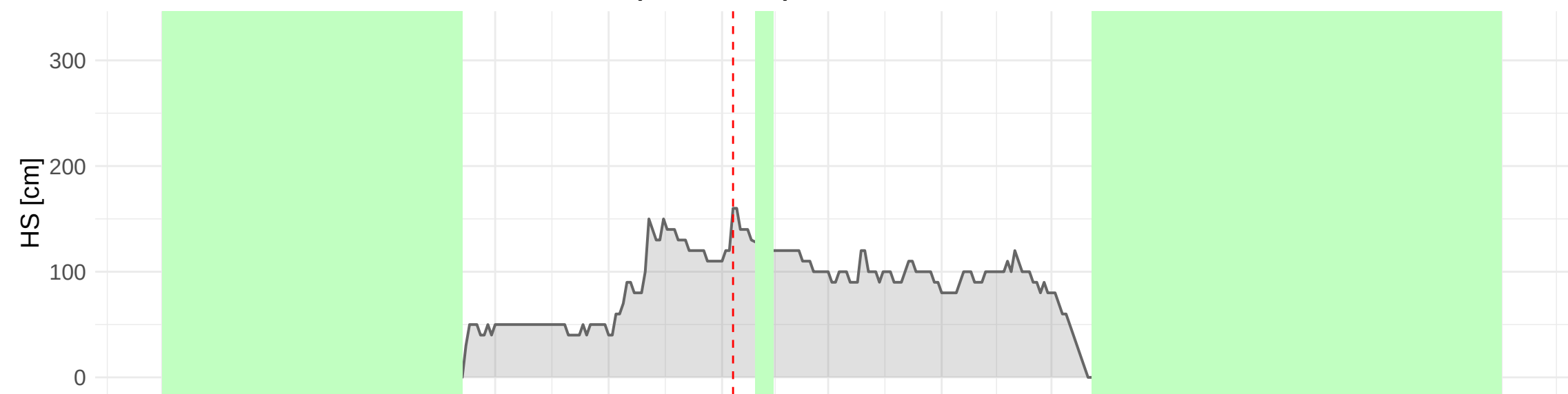
HSD_TAA_TN_DAONE_MALGA_BISSINA_MAN (1785 m a.s.l.) – 2007 to 2008
