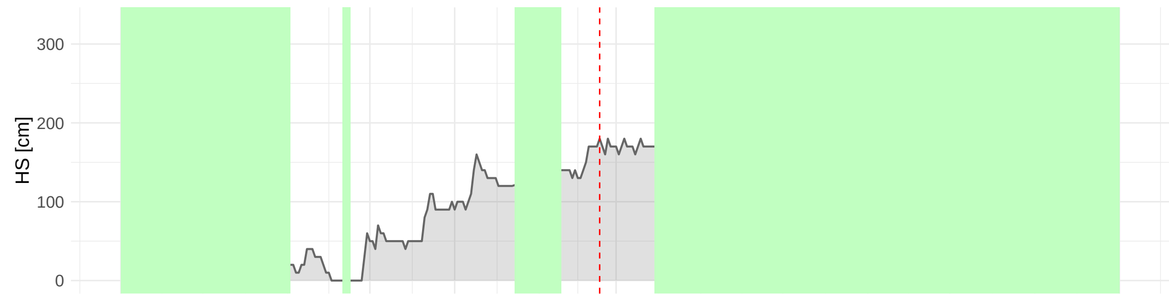
HSD_TAA_TN_DAONE_MALGA_BISSINA_MAN (1785 m a.s.l.) – 2009 to 2010
