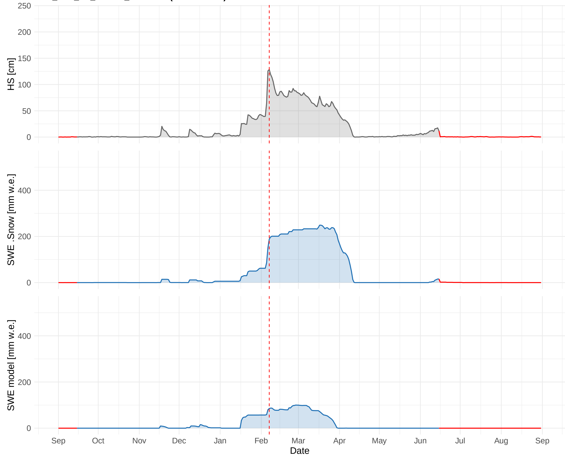
HSD_TAA_TN_PASSO_BROCON (1610 m a.s.l.) – 2014 to 2015
