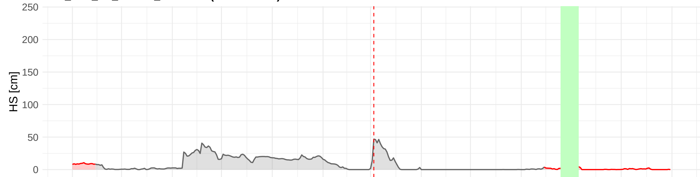
HSD_TAA_TN_PASSO_BROCON (1610 m a.s.l.) – 2019 to 2020
