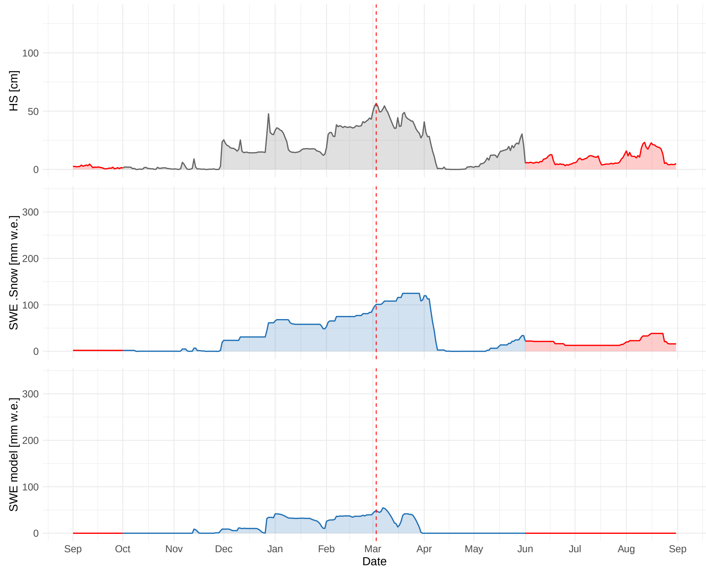
HSD_TAA_TN_PASSO_SOMMO (1360 m a.s.l.) – 2017 to 2018
