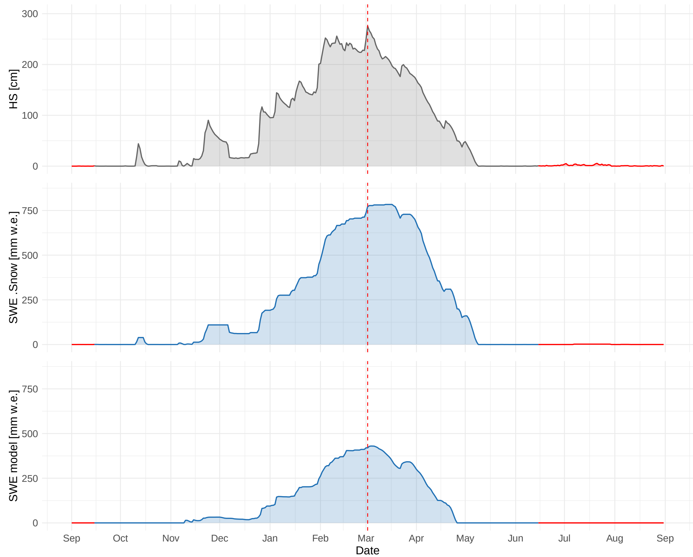
HSD_TAA_TN_PASSO_TONALE (1875 m a.s.l.) – 2013 to 2014
