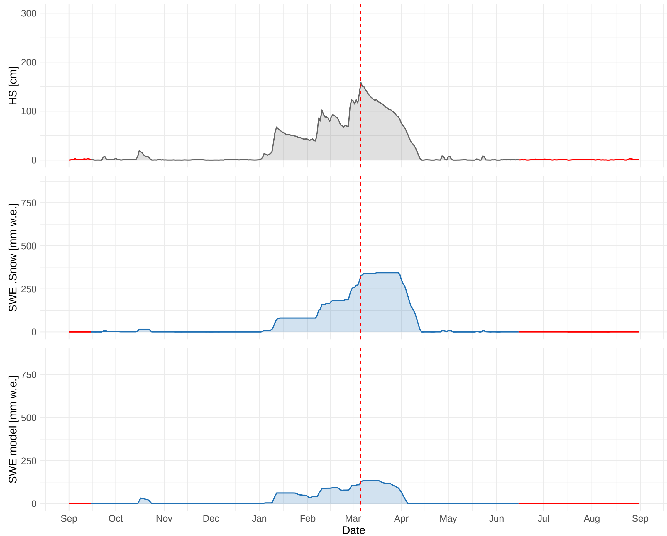
HSD_TAA_TN_PASSO_TONALE (1875 m a.s.l.) – 2015 to 2016
