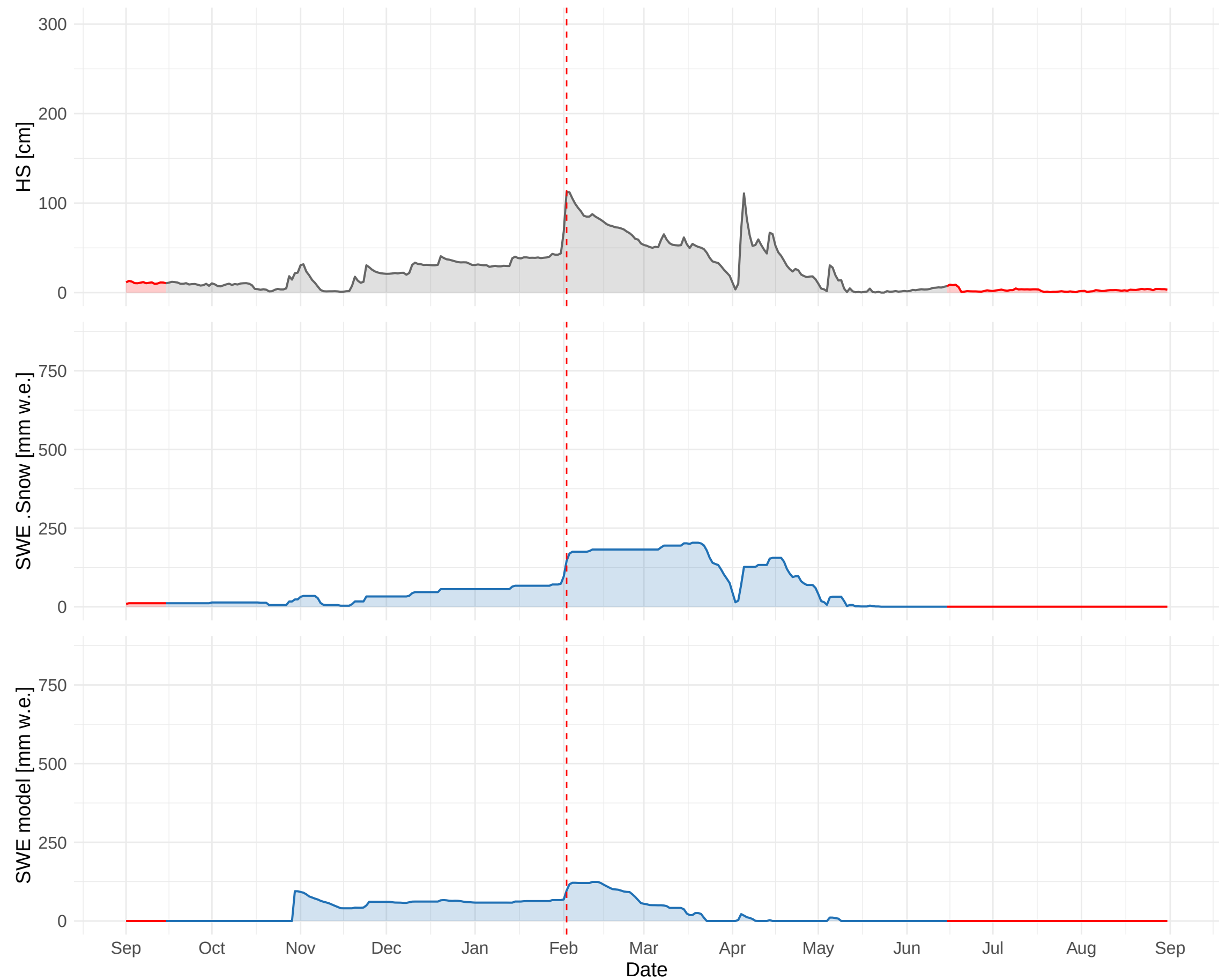
HSD_TAA_TN_PASSO_TONALE (1875 m a.s.l.) – 2018 to 2019
