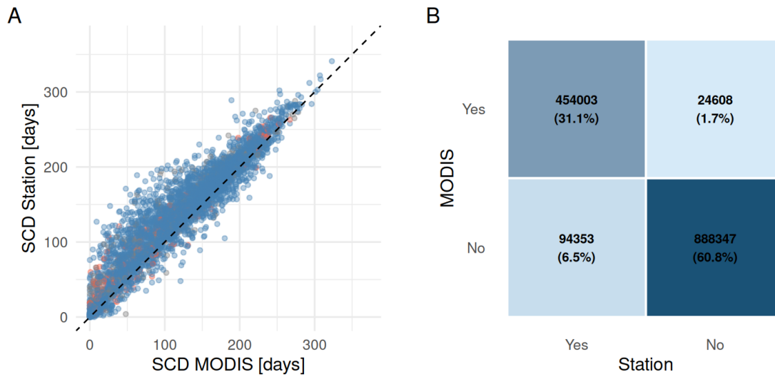
Figure 5.11: (a) Comparison between SCD values computed from HS series after correction and MODIS data. Each dot represents a pseudo-hydrological year, which is the period spanning from 1 September of a given year to 31 August of the following one. Blue dots are data retrieved from stations whose metadata are reliable, whereas orange ones are not. (b) Confusion matrix comparing snow presence according to MODIS and HS data.
