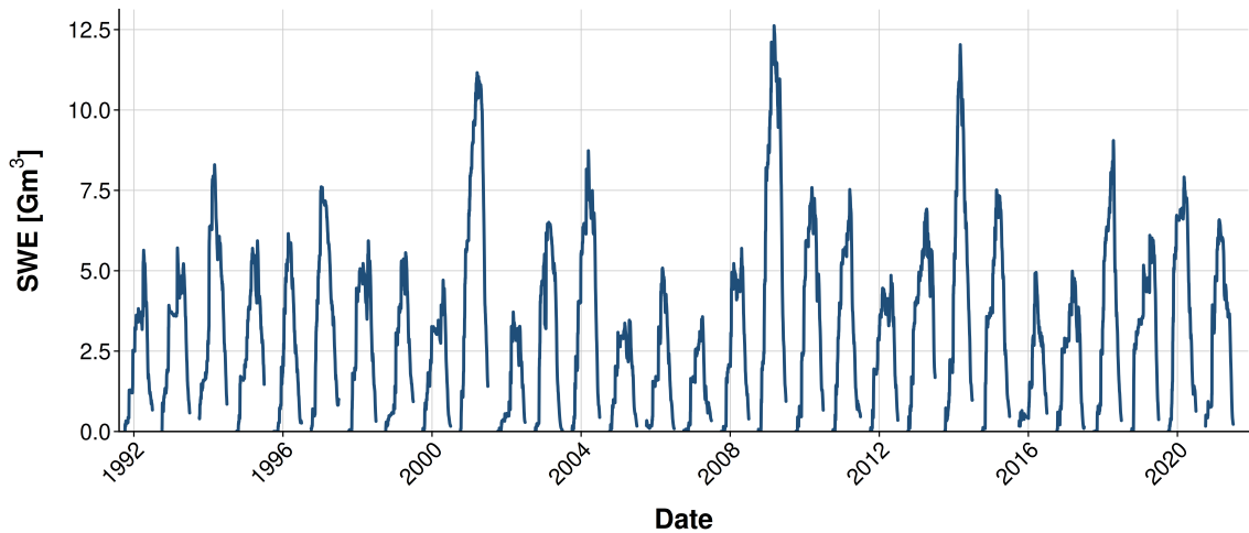
Figure 1.8: MODIS
