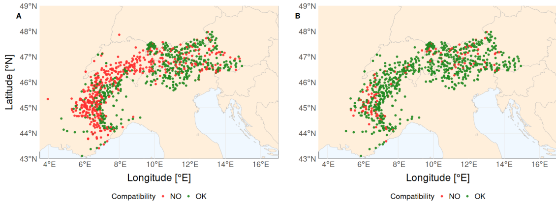
Figure 5.2: (A) Compatibility between declared station elevation and closest DEM point before checking station coordinates. (B) Compatibility between declared station elevation and closest DEM point after checking station coordinates. In both cases the ALOS AW3D30 global DEM was used: stations are labelled as compatible (OK) if the elevation difference is smaller than 12 m, namely 2/5 of pixel size.
