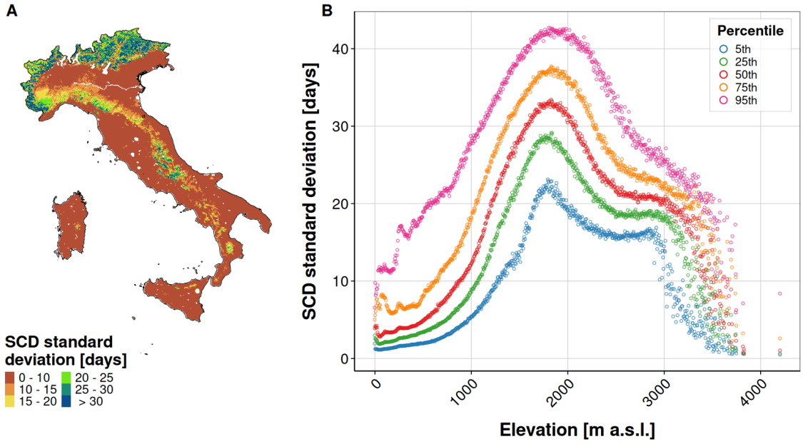
Figure 3.5: (a) Spatial distribution of SCD standard deviation from the mean, computed over the 2001-2025 period. (b)
