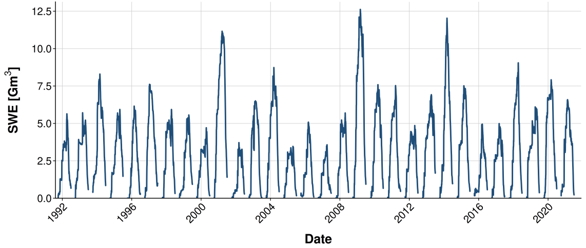
Figure 3.8: Daily evolution of the total water volume stored within the snowpack in the mountainous portion of the Po River District. The investigated period spans from 3 October 1991 to 1 July 2021. Data are from the Po River District snow dataset (Wani et al. 2025)
