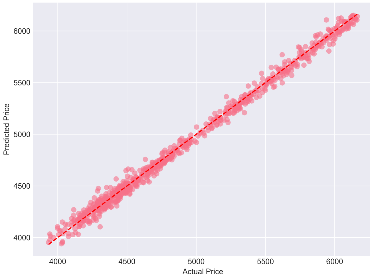
Actual vs Predicted Scatter Plot
