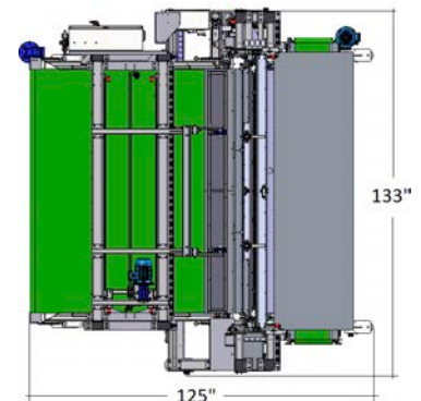
Footprint Vista Superior
