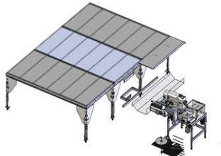
11339HFP82T with triple air table Con mesa de aire triple
