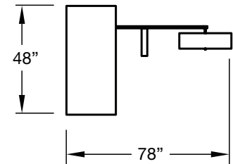
Footprint Vista Superior
