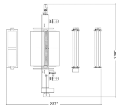
Footprint with winder/unwinder Visa Superior con enrollado/desenrollado
