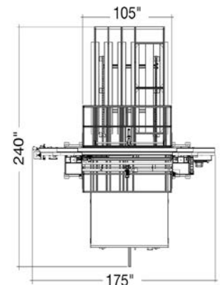
Footprint / Visa Superior 11385-X & X-O
