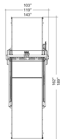
Foot print / Vista Superior
