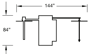
Footprint Vista Superior
