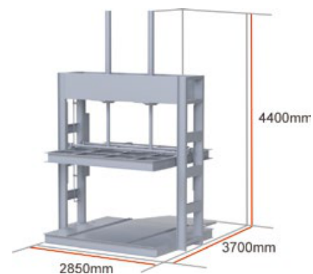
MACHINE SIZES
