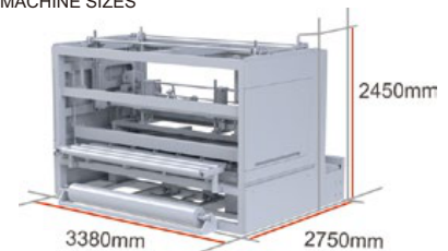
MACHINE SIZES
