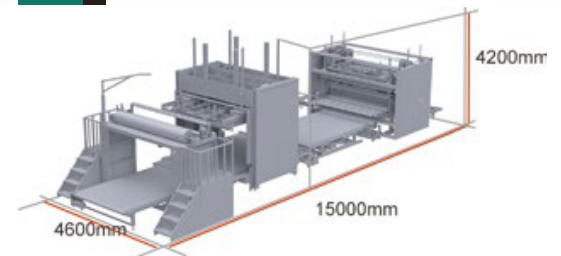
MACHINE SIZES
