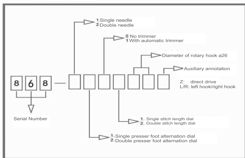
Code diagram
