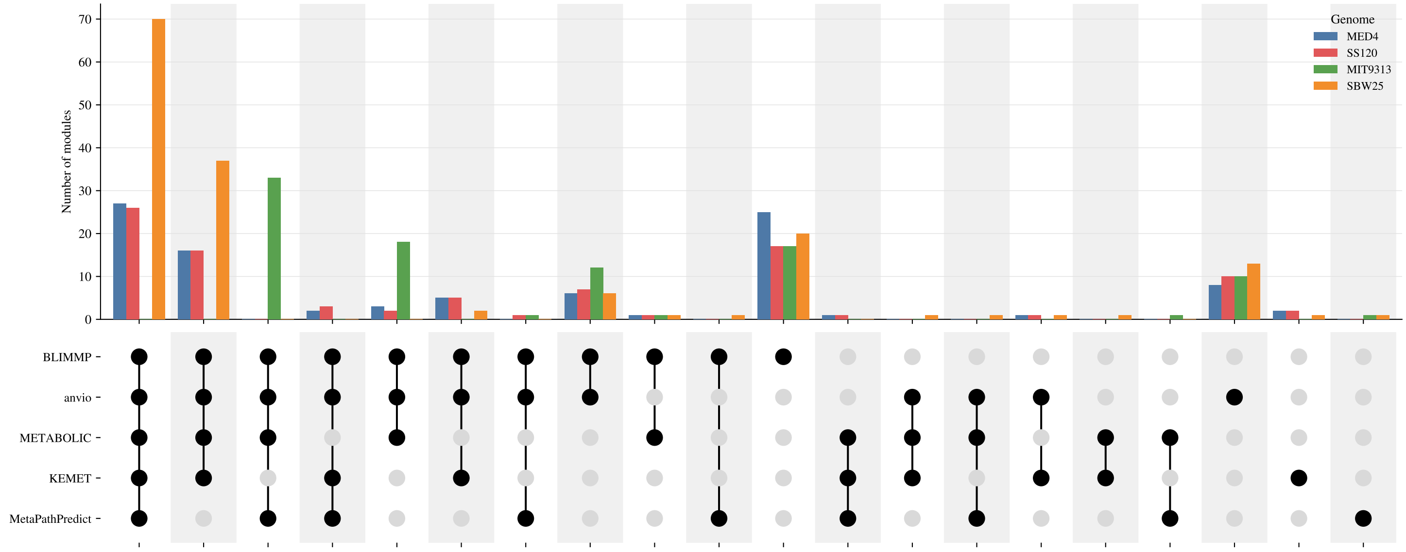
Tool agreement on module presence, by genome (0% gene removal) BLIMIMP-containing combinations first (most tools to fewest), then others; combinations with zero modules in every genome excluded
