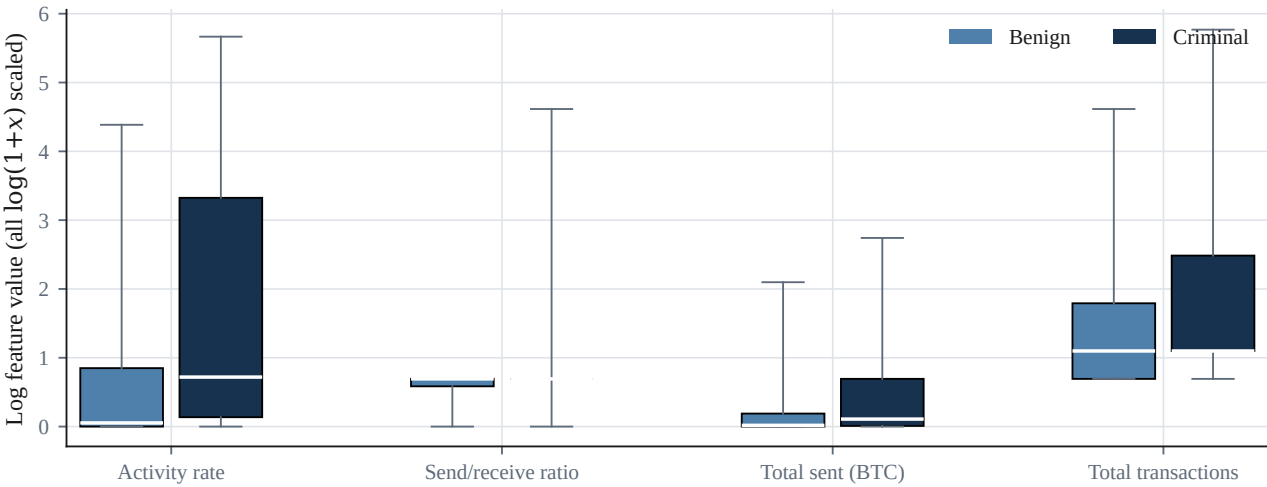
Class-conditional feature distributions (training corpus)
