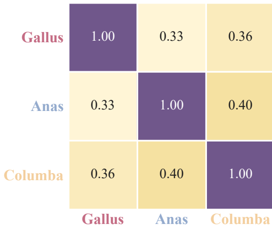
Jensen-Shannon
