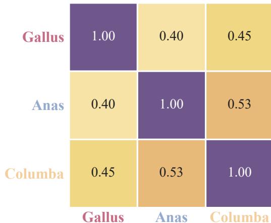
Bray-Curtis
