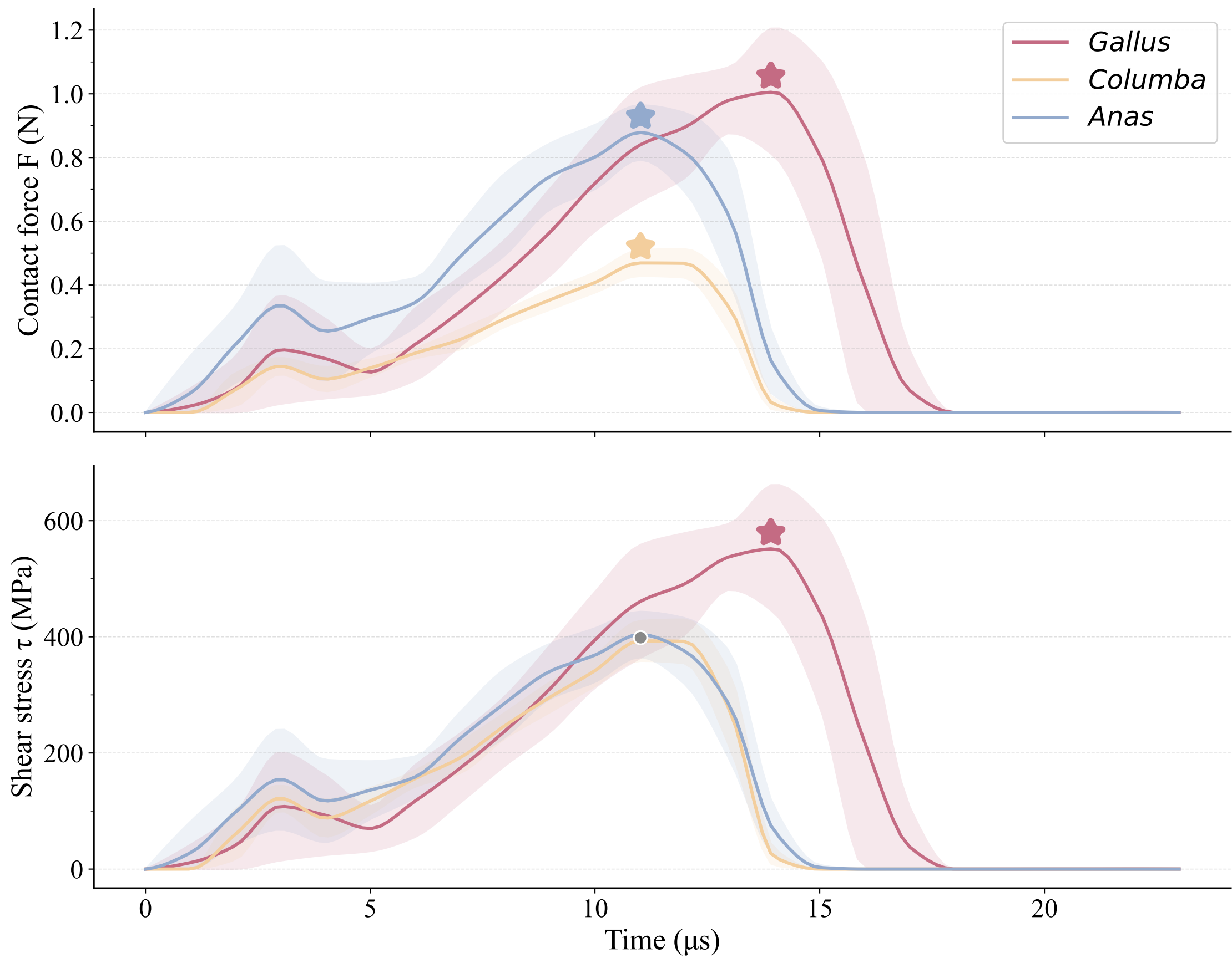
Contact Force and Shear Stress — Mean \pm 1\sigma across 9 impact positions
