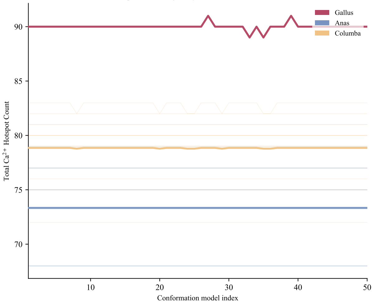
Hotspot Count Trajectory Across 50 Conformations
