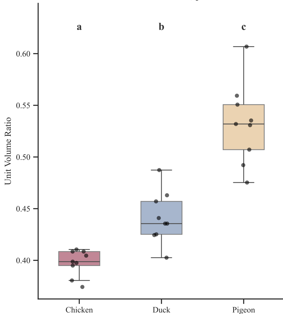
Unit Volume Ratio Duncan ANOVA: F=55.43 , p=1.01e-09
