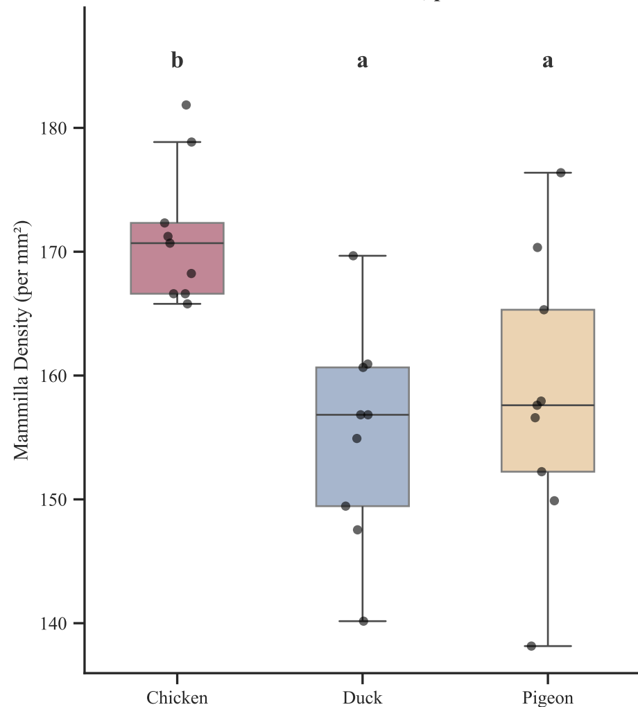
Mammilla Density Duncan ANOVA: F=8.41 , p=1.71e-03
