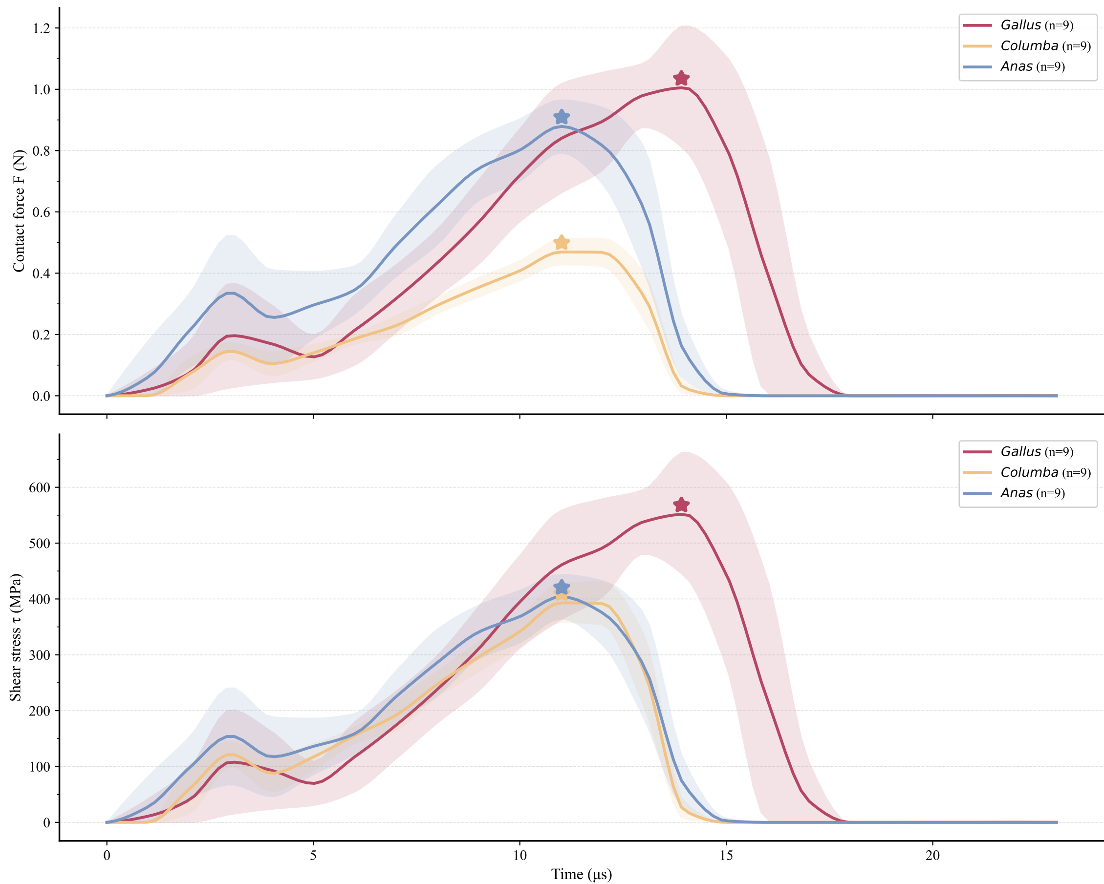
Contact Force and Shear Stress — Mean \pm 1\sigma across 9 impact positions
