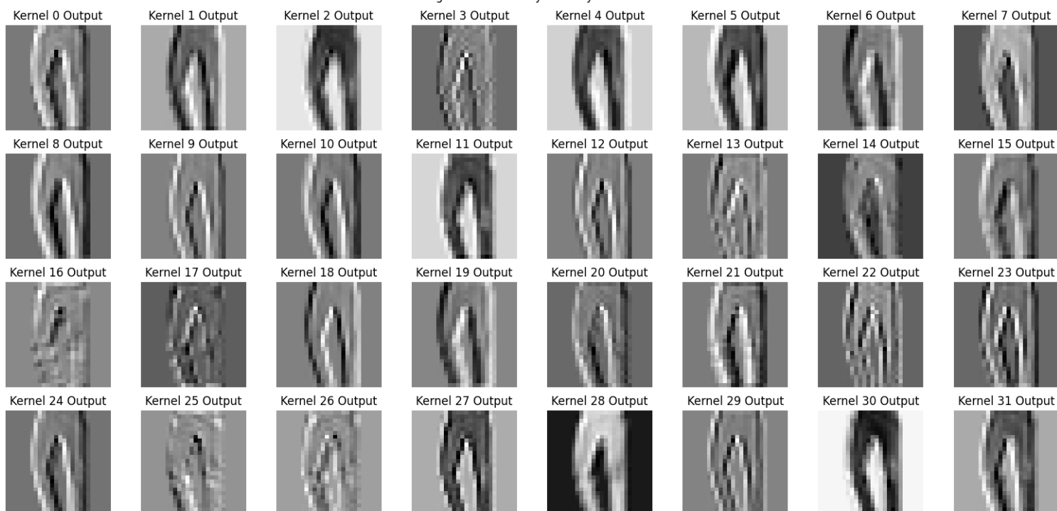
Image Transformed by First Layer Kernels
