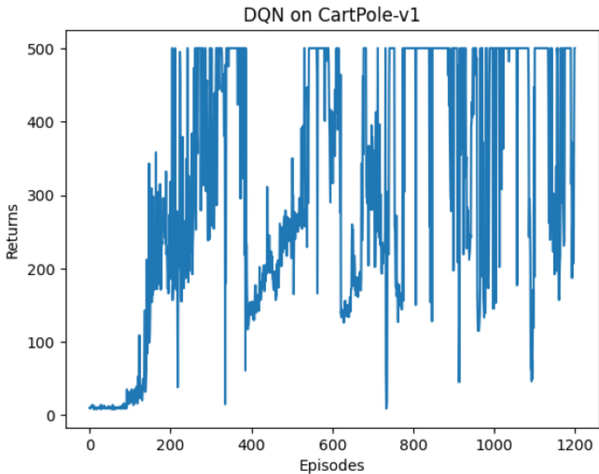
DQN training curve
