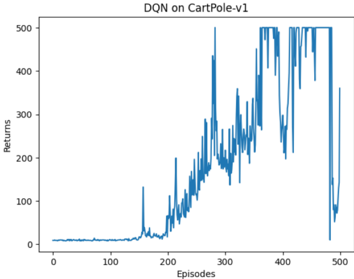
DQN training curve (CartPole)
