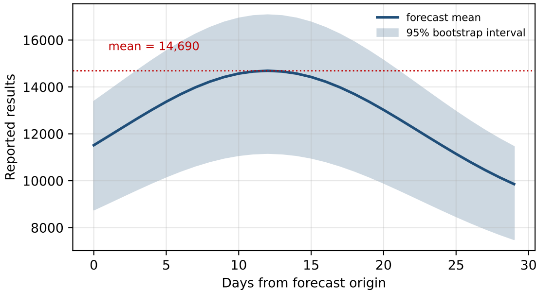
Bootstrap forecast with 95% interval
