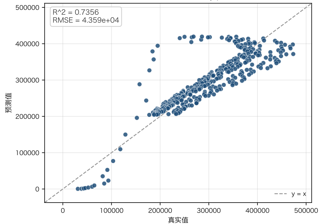
Predicted versus observed daily post volume
