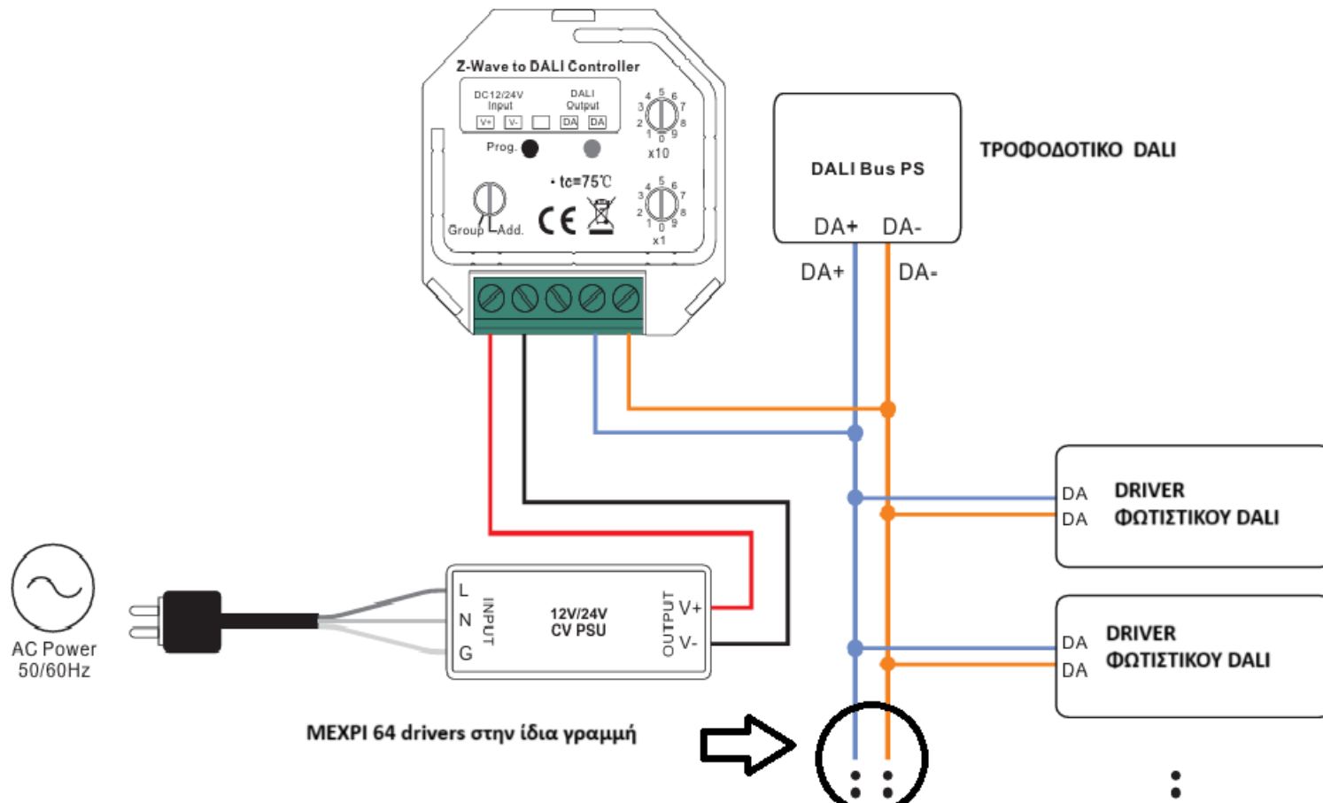
Wiring Diagram
