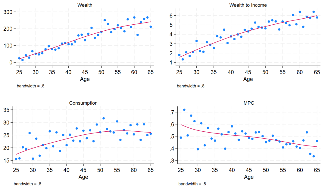
Figure G1: Life Cycle Profile of Consumption, MPC, and Wealth
