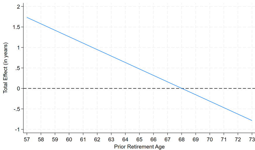
Figure 6: Treatment Effect as a Function of the Prior
