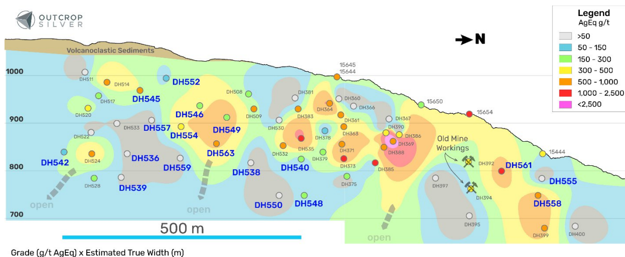
Figure 2. Longitudinal section from the Aguilar vein showing the drilling pierce points. The contours represent the interpolation of grade (AgEq g/t) multiplied by estimated true width (metres) using the Spline algorithm in QGIS. Pierce points and channel samples are showing grade as AgEq g/t.
