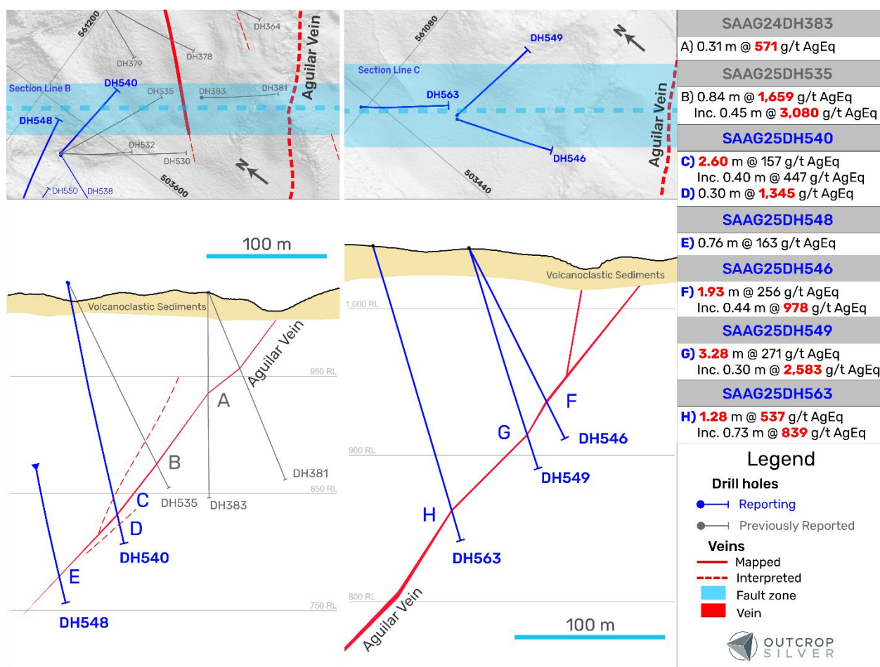
Figure 4. Geological cross-sections showing the Aguilar vein system. Cross-section B's width is 50 metres. Cross-section C's width is 75 metres. The lengths are downhole and do not represent estimated true widths.
