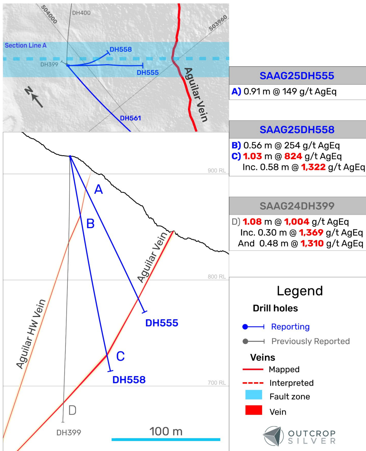
Figure 3. Geological cross-section A showing the Aguilar vein system. The cross-section's width is 35 metres. The lengths are downhole and do not represent estimated true widths.
