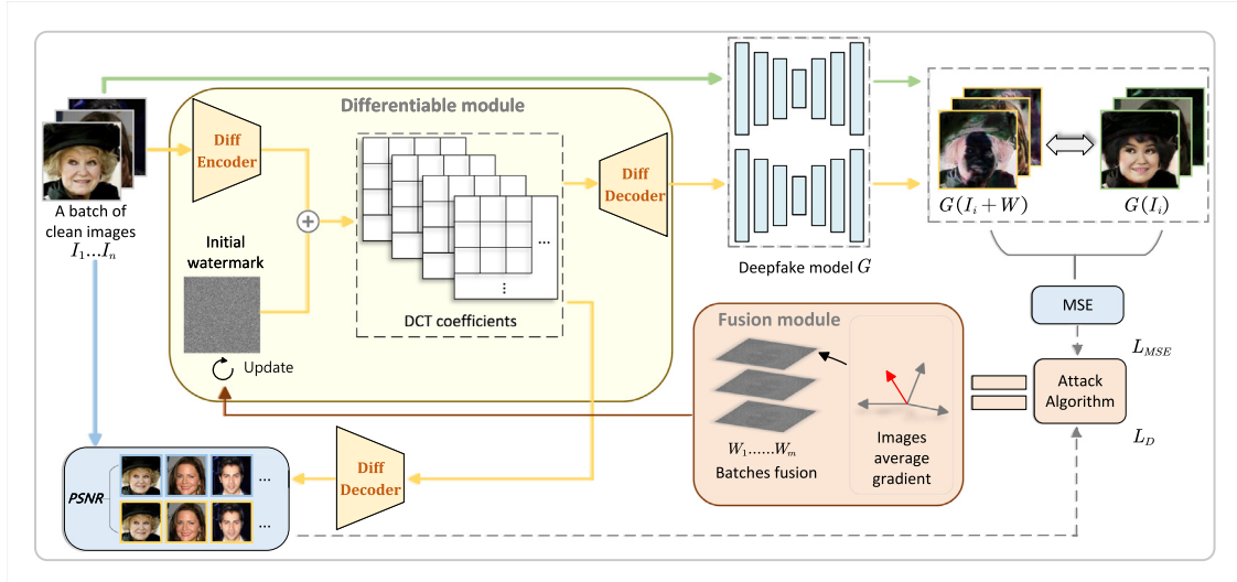
Fig. 2. The overall pipeline of our robust cross-image adversarial watermark defending against Deepfake models.
