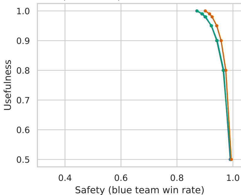
sharp honest UM, \rho = 0.0 (honest FPR = 0.007)
