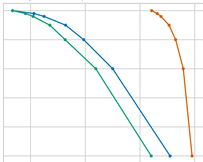
noisy honest UM, \rho = 0.6 (honest FPR = 0.160)
