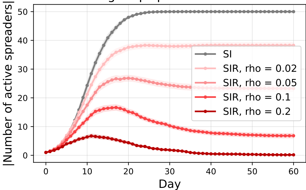
Active gossip spreaders over time
