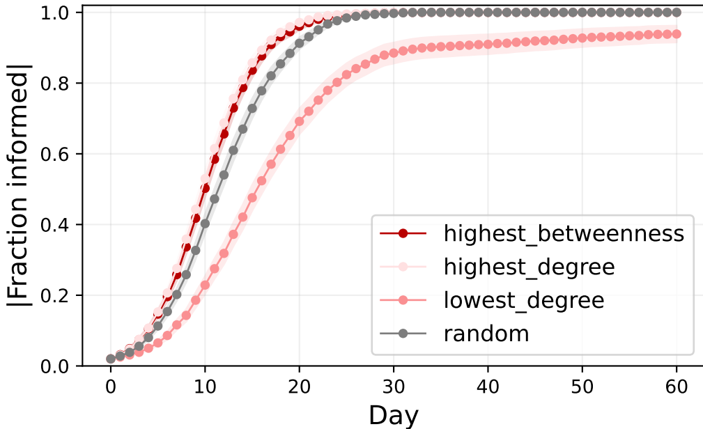
Effect of initial source on gossip spreading
