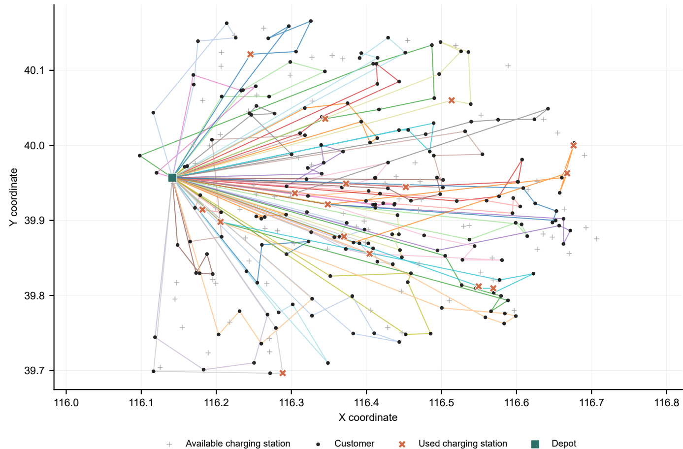
Representative EVRPTW-SPD solution | seed 42 | 44 vehicles | cost 70,113.56
