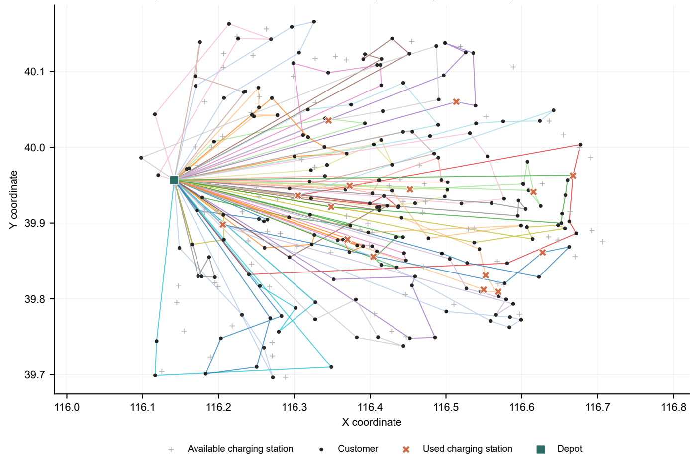
Representative EVRPTW-SPD solution | seed 45 | 45 vehicles | cost 72,526.86
